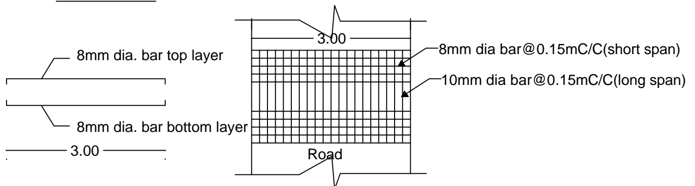
TYPICAL PLAN OF REINFORCEMENT
