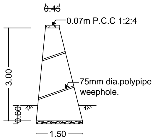
SECTION OF RETAINING WALL
