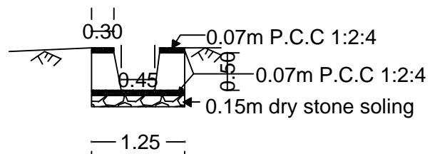
TYPICAL SECTION OF SIDE DRAIN
